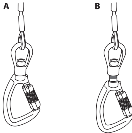
Figure 13: Inspecting SRL Load-Indicating Leg-end Connector A Regular Safe Operating Condition of Swivel Leg-end Connector B Visual Indicator Exposed on Connector - Remove SRL from Service
