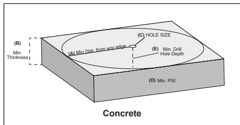
FIGURE 6 - INSTALLATION SPECIFICATIONS DIAGRAM
