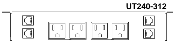
UT240-312 UT240-410 Europe UT240-450 England UT240-510 Australia UT240-550 Universal * The circuit breaker is located on the inside of the left-hand side of each unit as viewed from the front. (see Diagram 14) AC (4) Net (4) Circuit Breaker (1)
