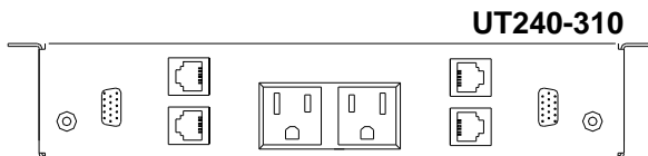
UT240-310 UT240-411 Europe UT240-451 England UT240-511 Australia UT240-551 Universal AC (2) VGA (2) Net (4) Audio (2)
