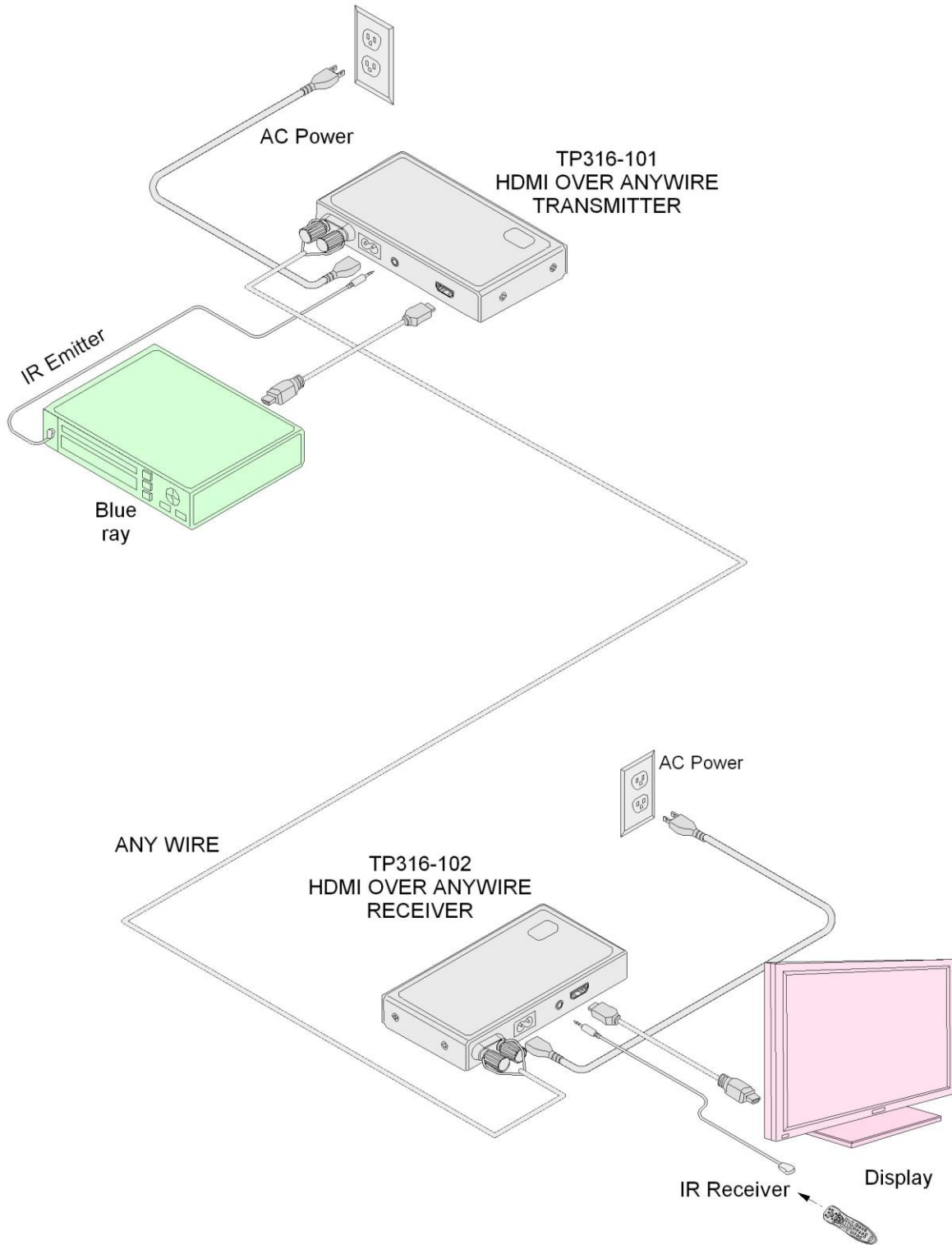
Diagram 1: Typical Setup
