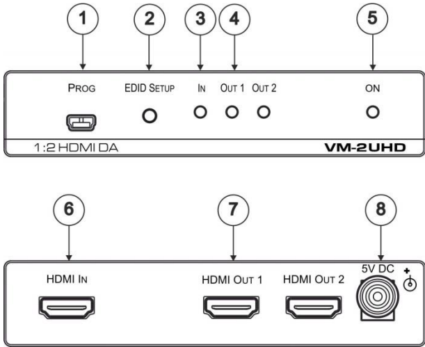
Figure 1: VM-2UHD 1:2 HDMI DA
