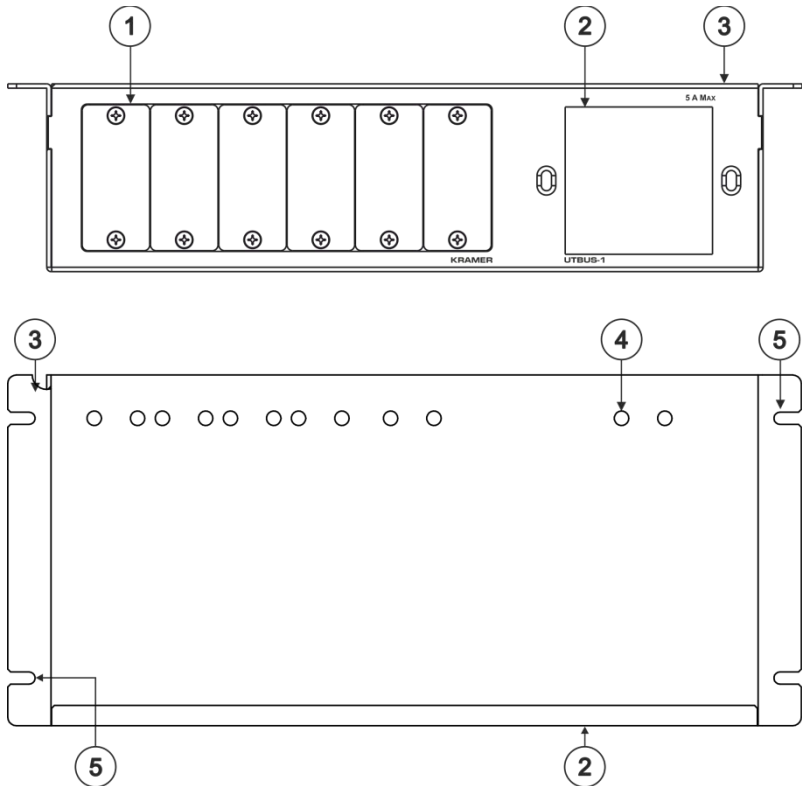
Figure 2: UTBUS-1xl Under the Table Connection Bus
