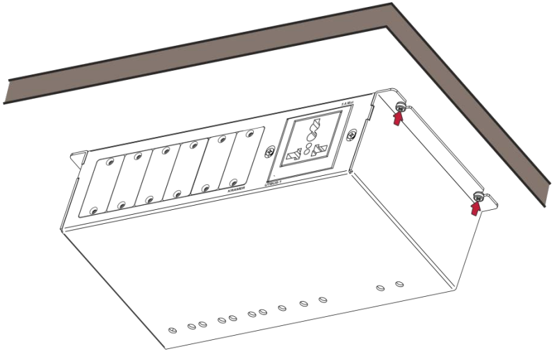
Figure 4: Securing the UTBUS-1xl Under the Table
