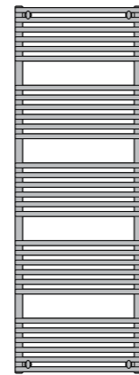
1738mm 30 Cross Bars
