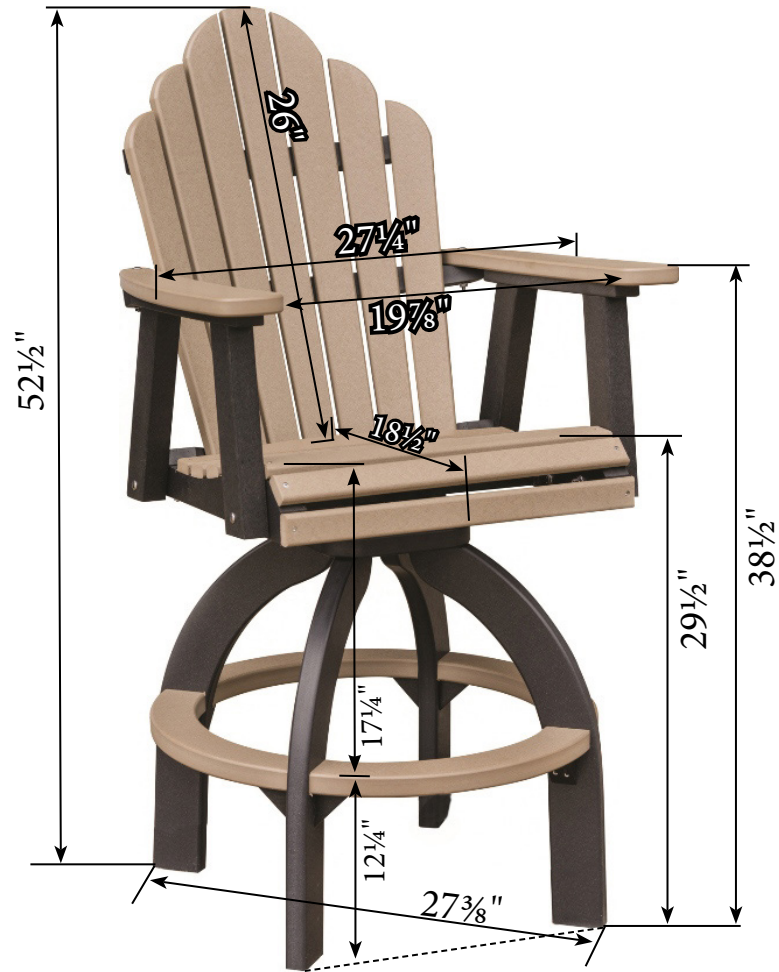
Cozi-Back Swivel 30'' XT Chair
