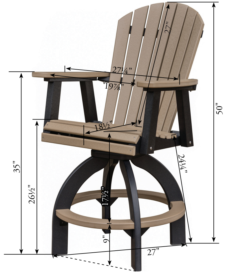
Comfo-Back Swivel Bar Chair
