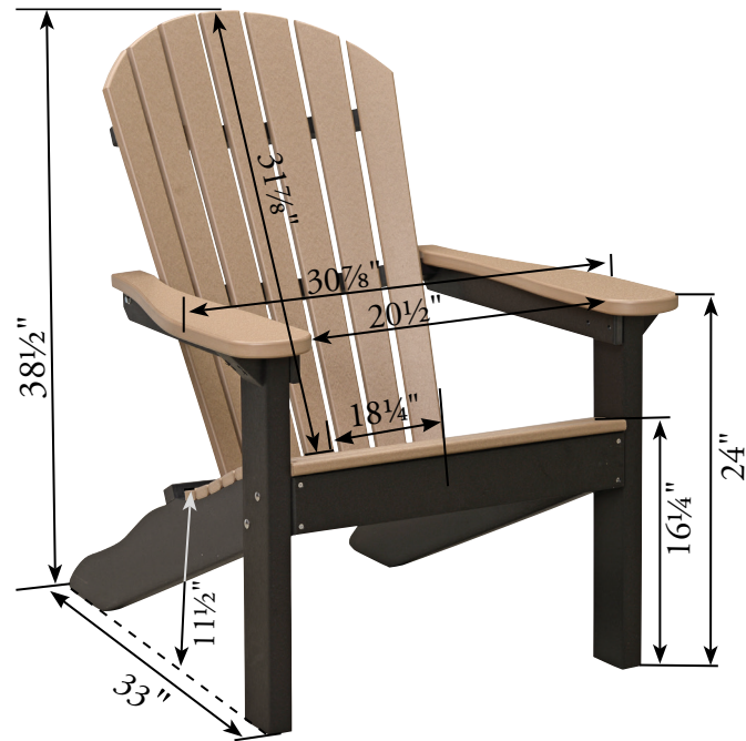
Comfo-Back Adirondack Chair
