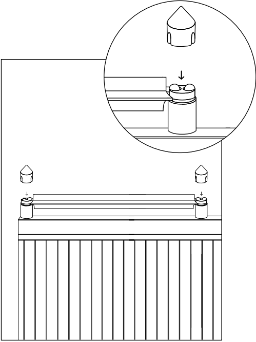
STEP 14 Place a cap (2) on each post.
