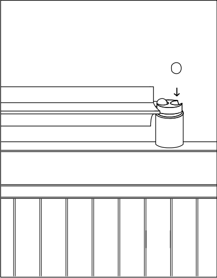
STEP 13 Place a ball in the second knuckle indent of the last post that you installed.
