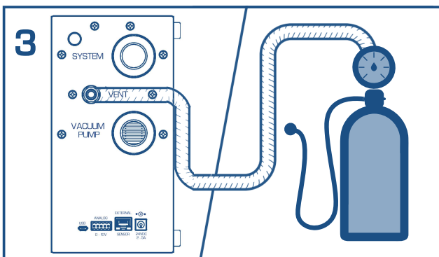
3 (Optional) Connect vent house to nitrogen or other inert gas or leave open to air
