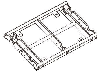
Stack Frame ZETHUS-SF1 (Fit ZETHUS-208(210)/ZETHUS-218S)
