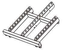
Flying Frame ZETHUS-115SFF (Fit ZETHUS-115S) (Fit ZETHUS-208) (Fit ZETHUS-110 with Adaptor A) (Fit ZETHUS-205 with Adaptor B)
