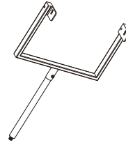
Support Stand ZETHUS-205SS (Fit ZETHUS-110S/ZETHUS-205) ZETHUS-208SS (Fit ZETHUS-112S/ZETHUS-208) One end with M20 bolt.
