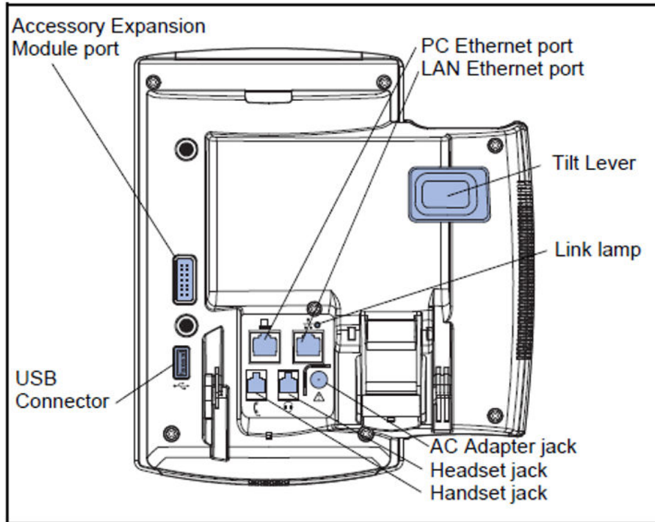
Figure 5: IP Deskphone connections
