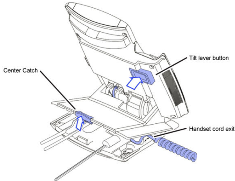
Figure 7: Remove the stand cover
