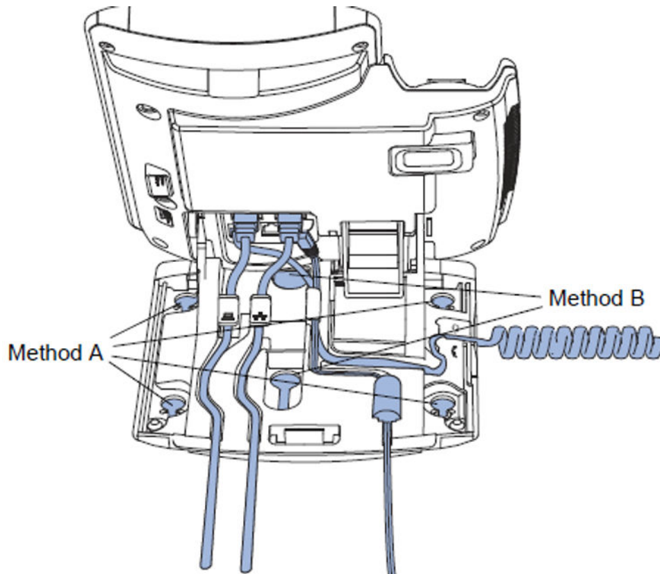
Figure 9: Cable routing tracks and mounting holes
