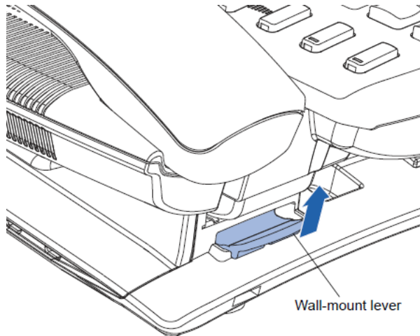
Figure 6: Wall-mount lever.
