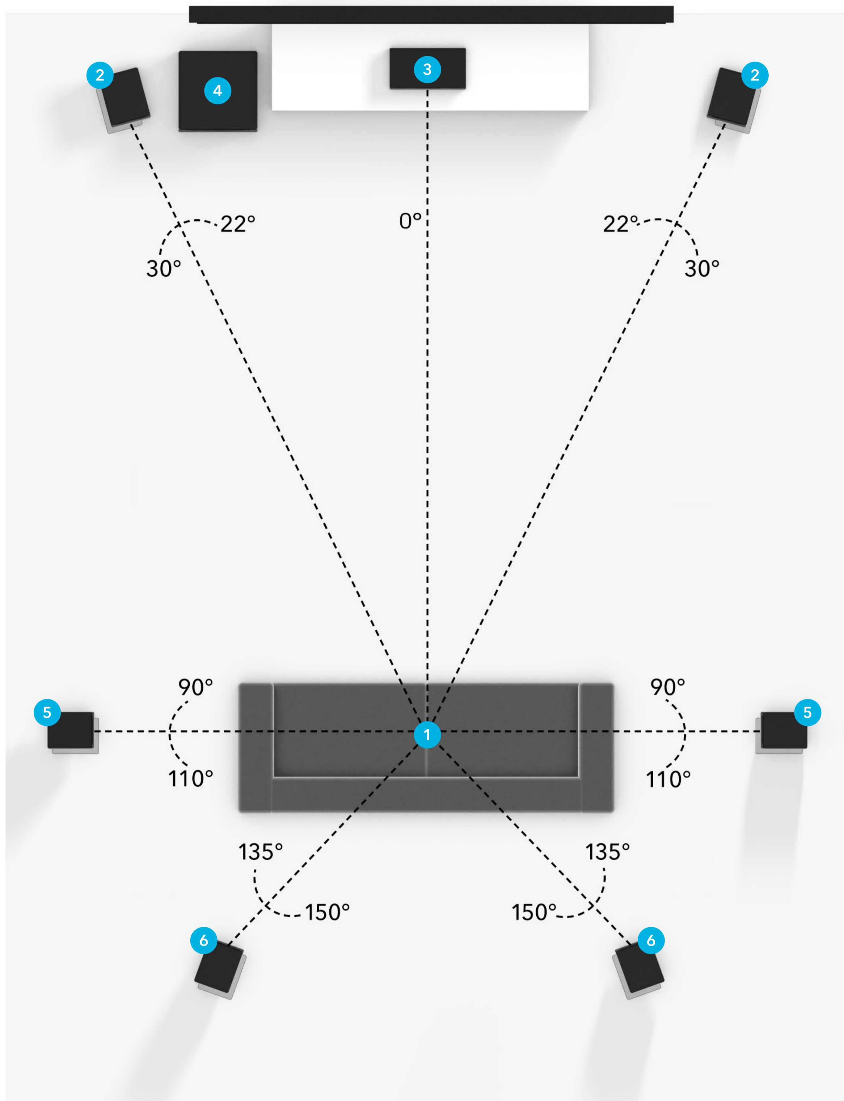
SPEAKER PLACEMENT FOR 7.1 SETUP
