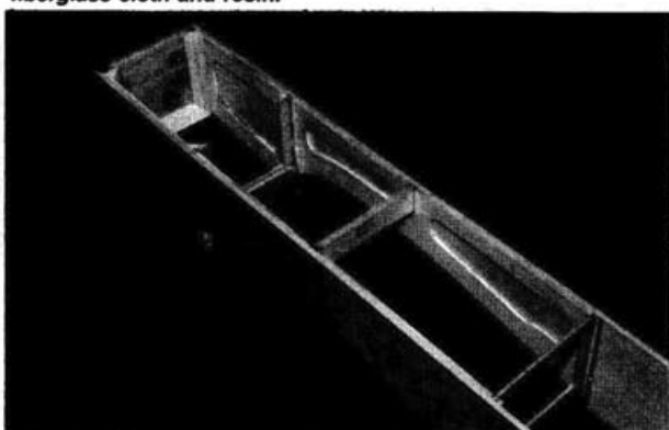
Assembly of the fuselage starts with the center formers and the firewall.
