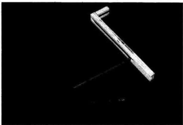
Plywood landing gear block and 3/16" music wire strut, ready to install in wing.
