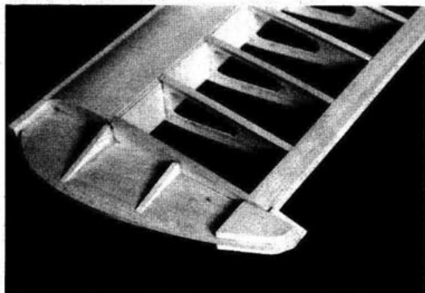
Wing tips and leading edge ready for sanding. Template was used to check leading edge contour.
