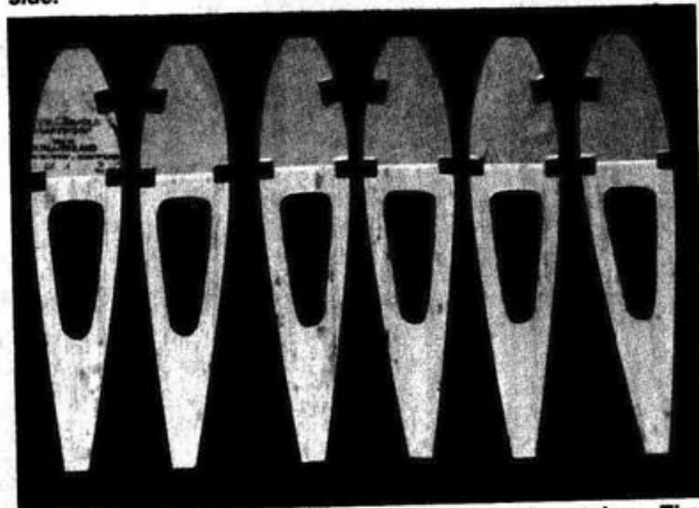
Ribs with plywood doublers and gear block notches. The lightening holes are optional.
