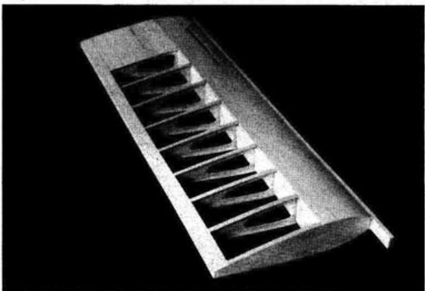
Sheeting and capstrips complete the wing panel. Note leading edge extension.
