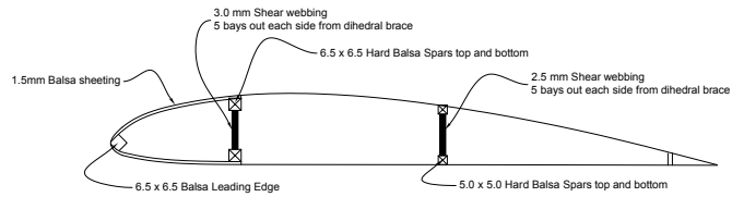
Modified Wing Construction
