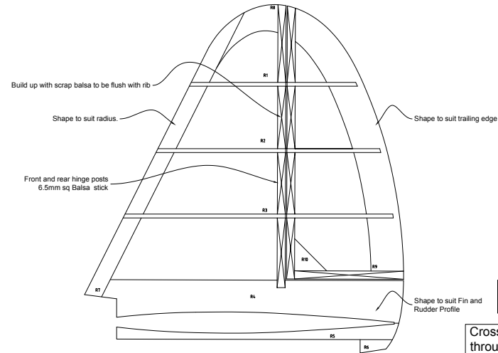
Modified Fin and Rudder Construction
