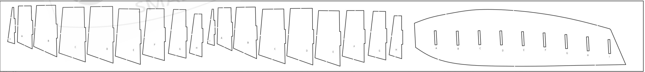
Float Base - This has been cut 1.5 mm undersize , so once you have glued it together, you can fill the spaces with foam blocks, shape and then cover with balsa and finally glass it to water proof it.
