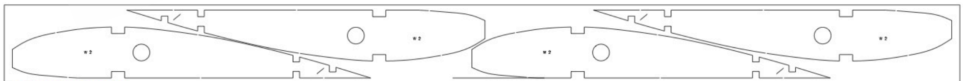
3.0 mm Balsa x 2
