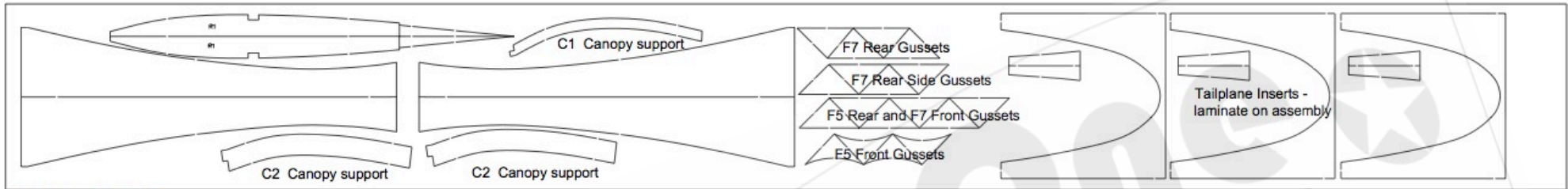
6.5 mm Balsa
