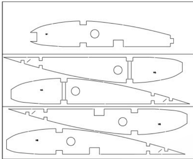
3.0 mm Poplar
