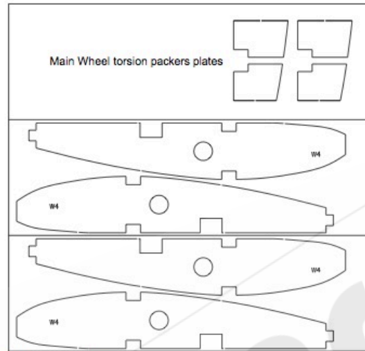
5.0 Bass mm Ply
