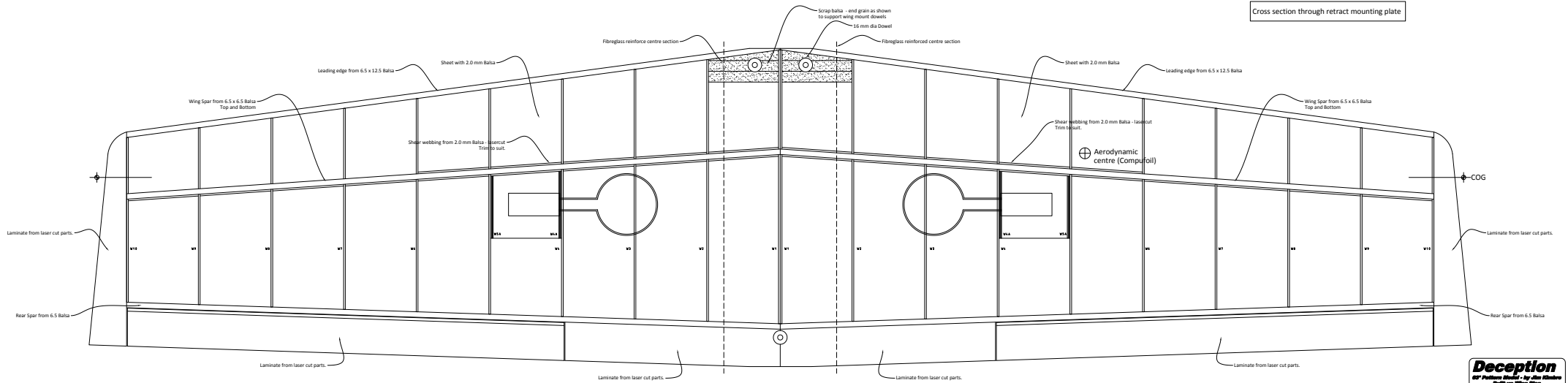
Cross section through retract mounting plate
