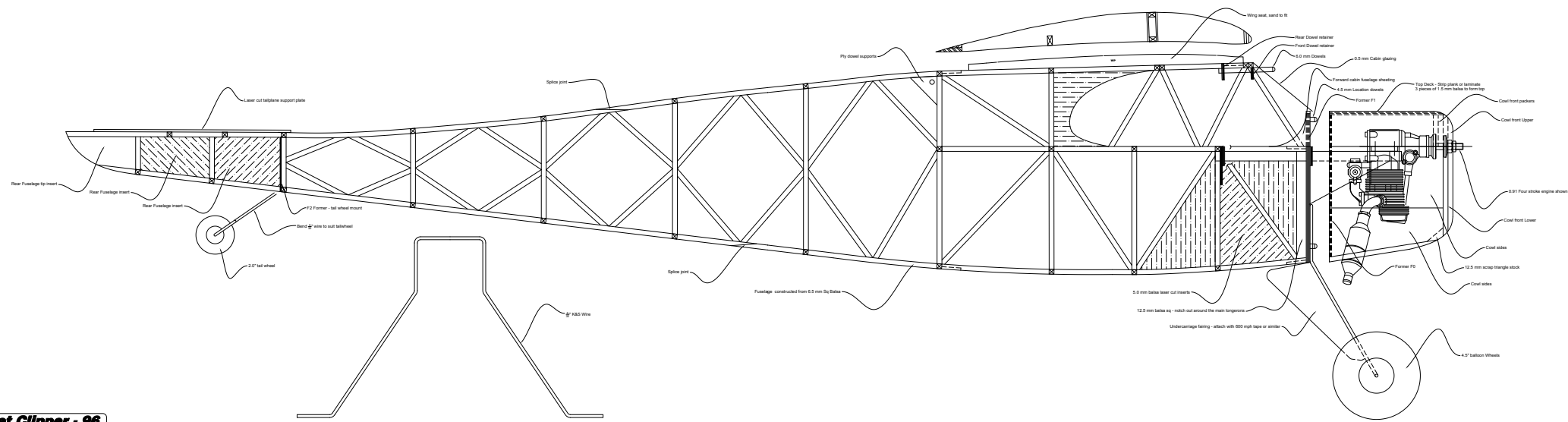
Comet Clipper - 96 Fuselage Plan
