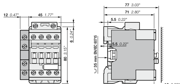
AF09, AF16 + CAL4-11 2-pole auxiliary contact block
