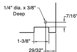
Undermount with hook hole boring
