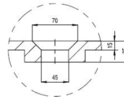
DETAIL D SCALE 1:3
