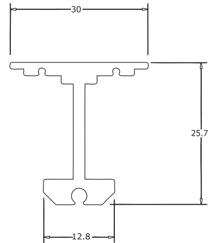
TRACK DIMENSIONS
