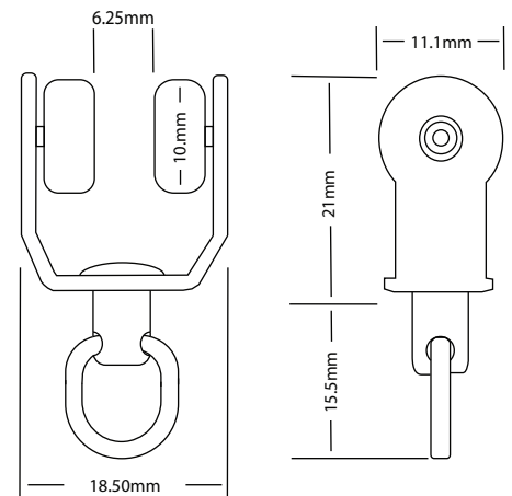
RUNNER DIMENSIONS
