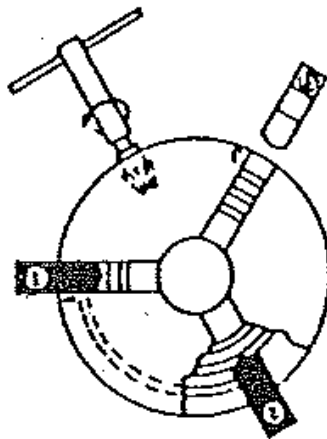
FIG#1, Steps in Mounting the Jaws
