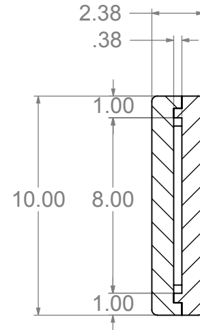
SECTION P-P
