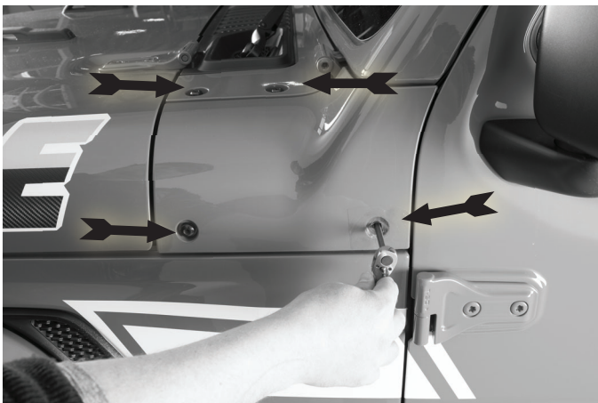
Fig 2 Remove the 4 T-40 torques head bolts from this body panel on the Jeep and remove body panel
