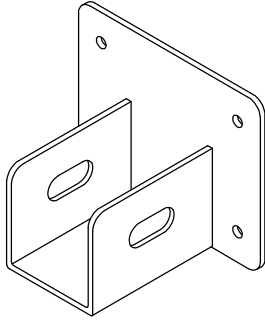
20674 (45*76*25mm)
