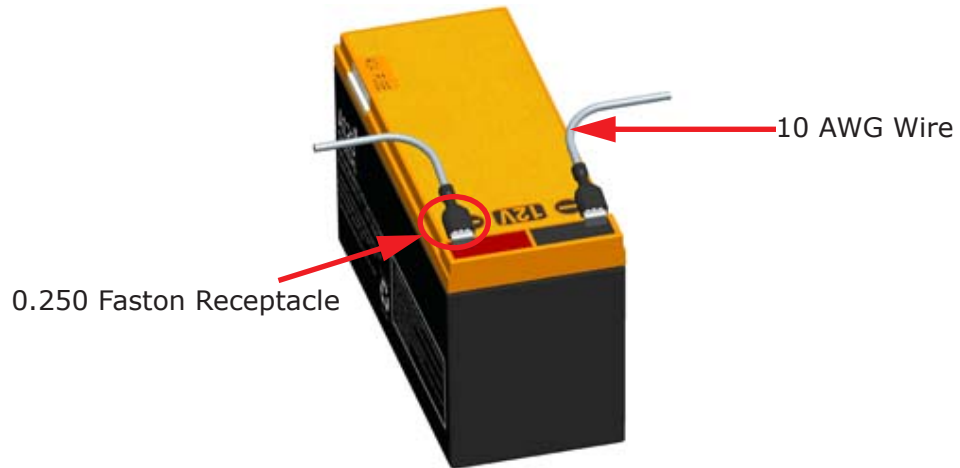
Figure 4-1 Components Used to Connect Multiple ALM 12V7s
