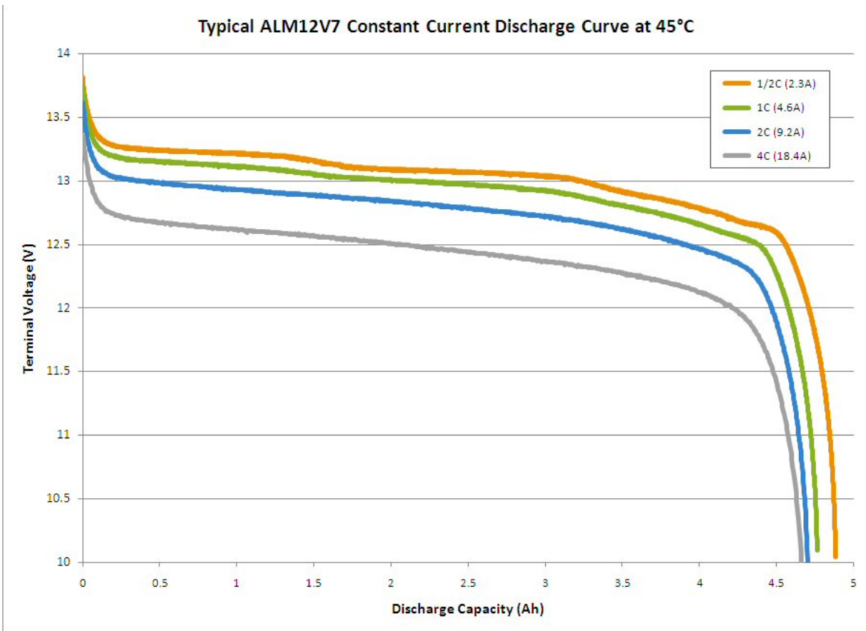
Figure 3-5 Discharge Curve at 45°C
