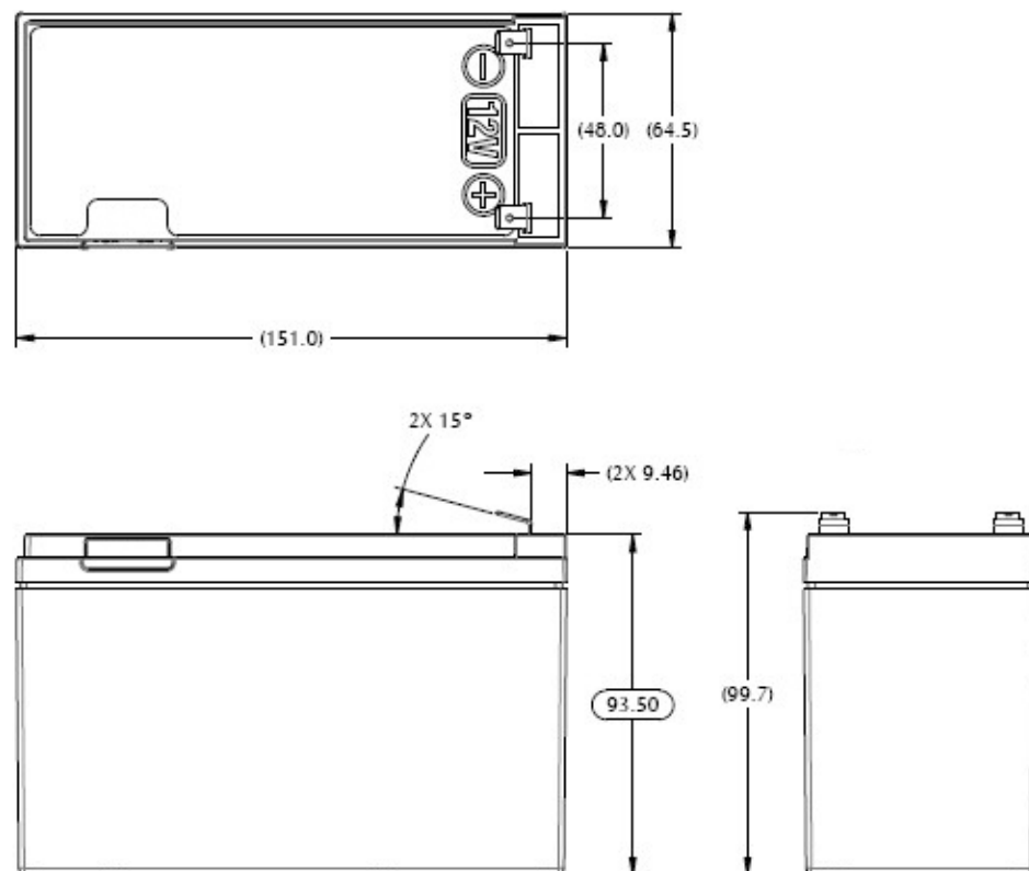
Figure 3-2 ALM 12V7 Mechanical Dimensions
