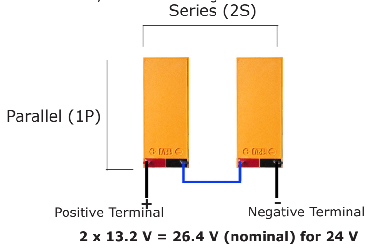
Figure 4-2 Connecting Batteries in Series (2S1P Configuration)
