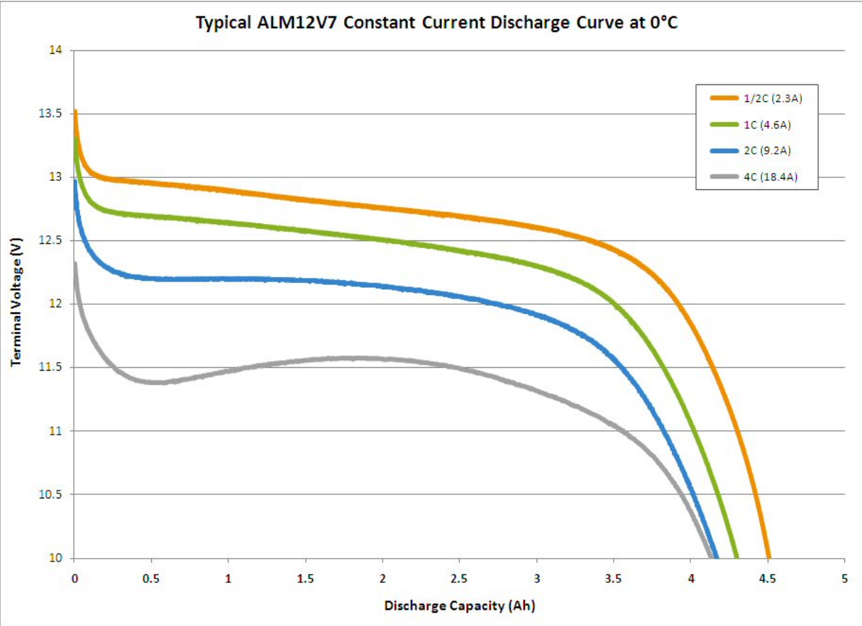
Figure 3-4 Discharge Curve at 0 °C
