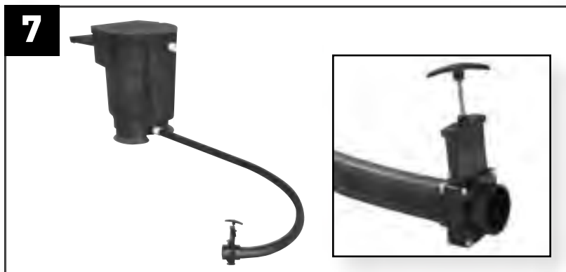
7 Glue the included knife valve to drain pipe end. Allow 20 minutes drying time.
