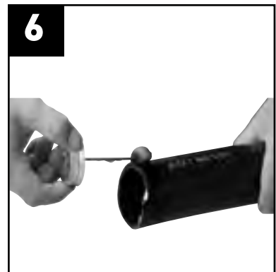
6 Glue the 5' section of 1.5" Savio Aqua Flex PVC™ to lower bulkhead.
