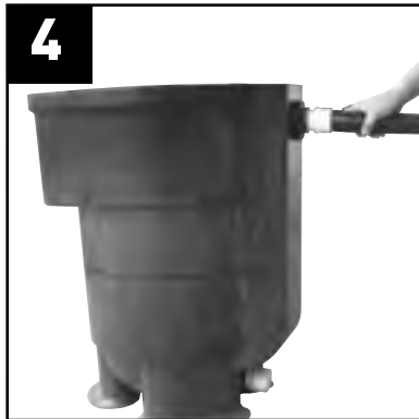
4 While glue is still wet, attach PVC to the male adapter.
