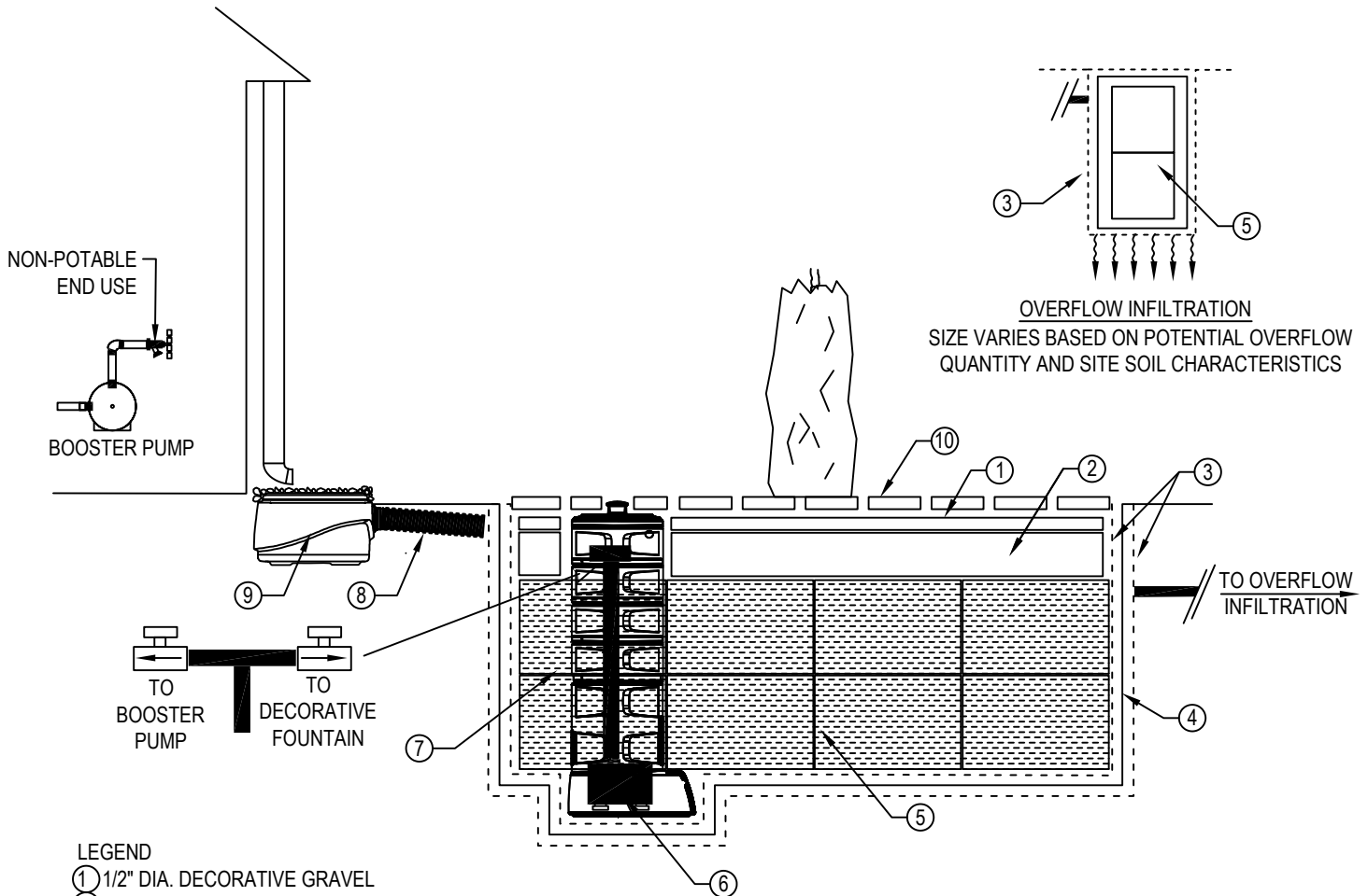
AQUA RAINWATER HARVESTING SYSTEM WATER FEATURE WITH PERMEABLE PAVER PATIO INSTALLATION
