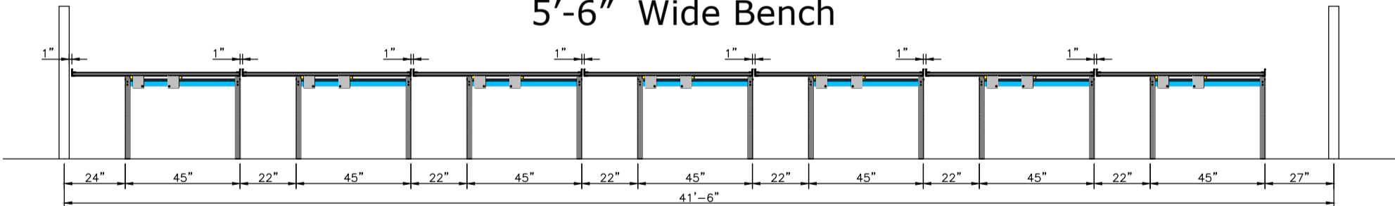
6' Wide Bench
