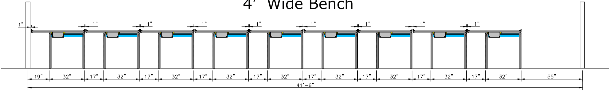
4'-6" Wide Bench
