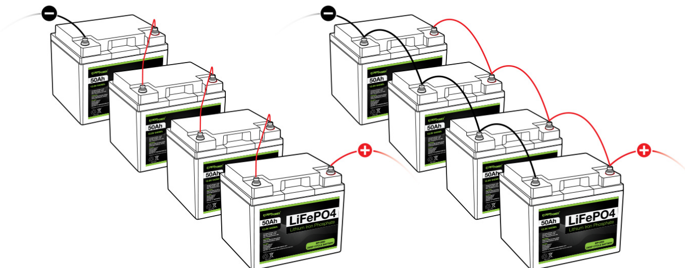
4 In Series - 48V 50Ah
