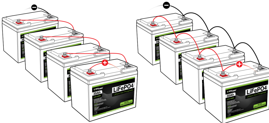
4 In Series - 48V 35Ah
