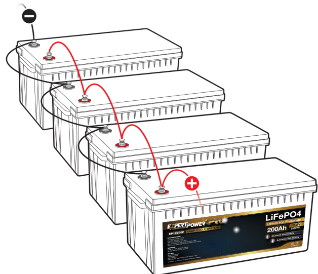
4 In Parallel - 12V 800Ah
