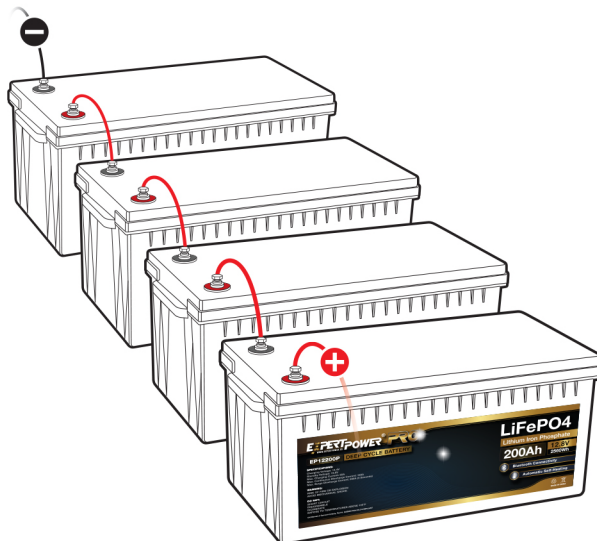
4 In Series - 48V 200Ah
