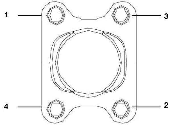
Figure #1 Bolt assembly order
