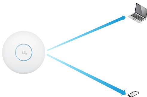
MU-MIMO with 3x3 and 1x1 clients: The UniFi SHD AP communicates with one 3x3 client and one 1x1 client at a time.
