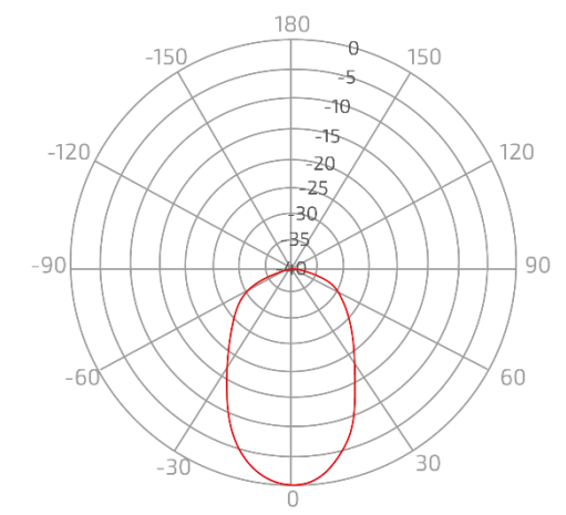
Elevation - SH-5800-18-30-DP
