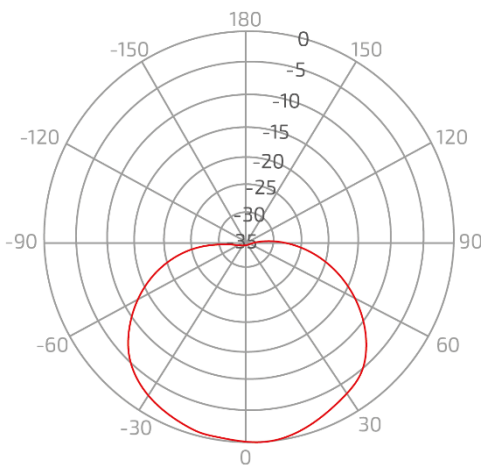
Elevation - SH-5800-10-90-DP
