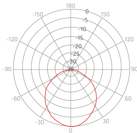
Azimuth - SH-5800-13-60-DP
