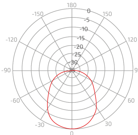
Elevation - SH-5800-13-60-DP
