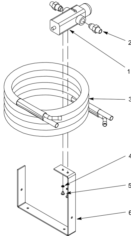
FIGURE 14. WATER COIL ASSEMBLY
