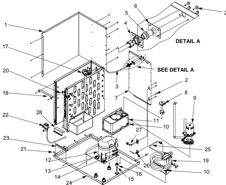
FIGURE 6. BUILD ASSEMBLY (WATER COOLED)
