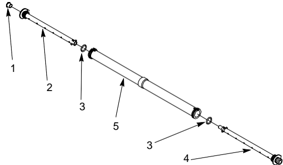
FIGURE 11. WATER DISTRIBUTOR ASSEMBLY
