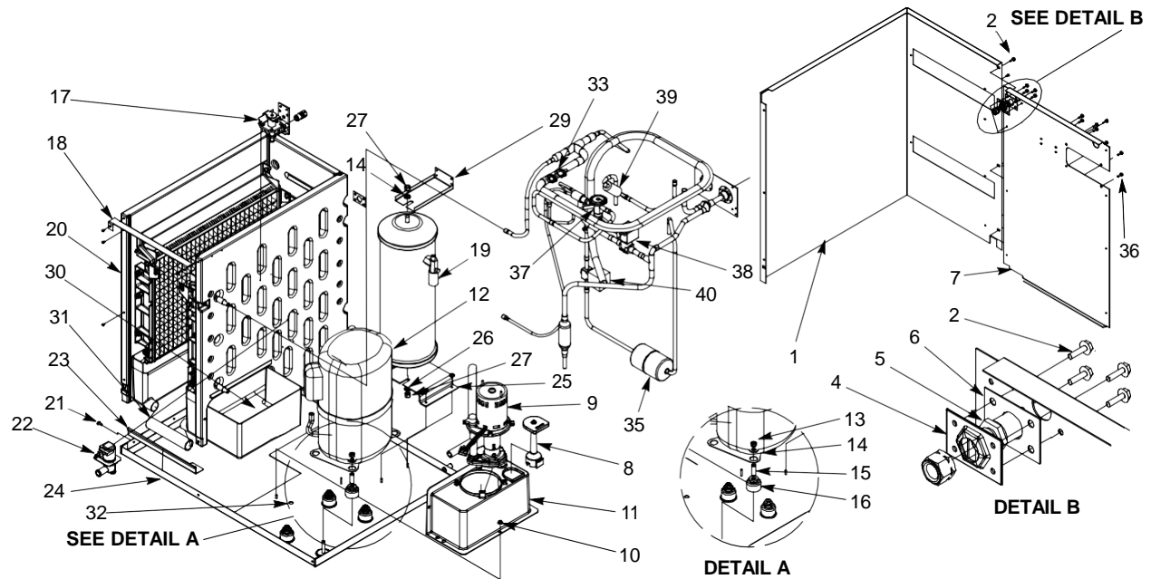
FIGURE 4. BUILD ASSEMBLY (REMOTE)
