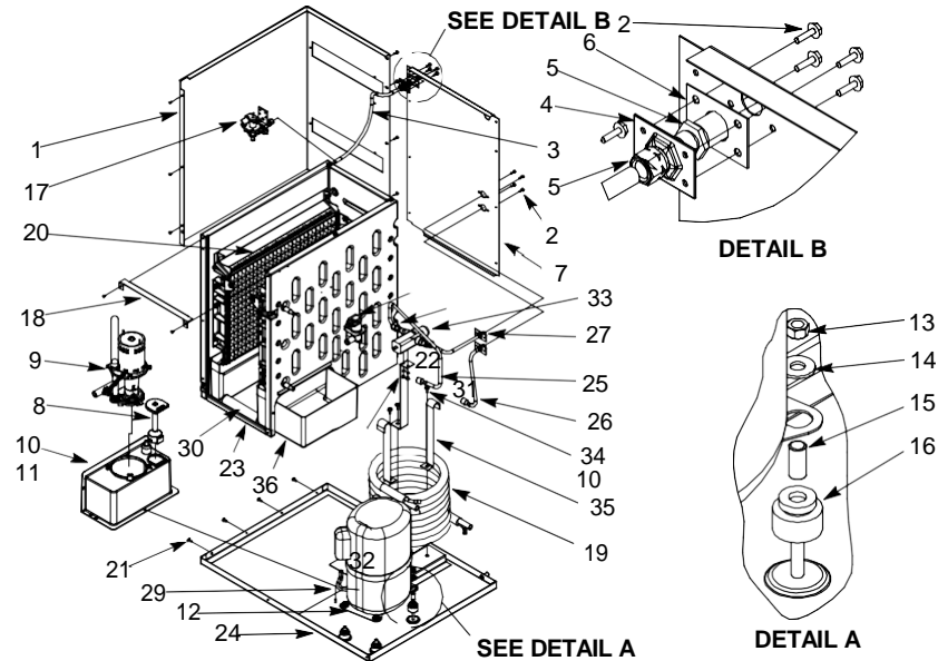
FIGURE 5. BUILD ASSEMBLY (WATER COOLED)
