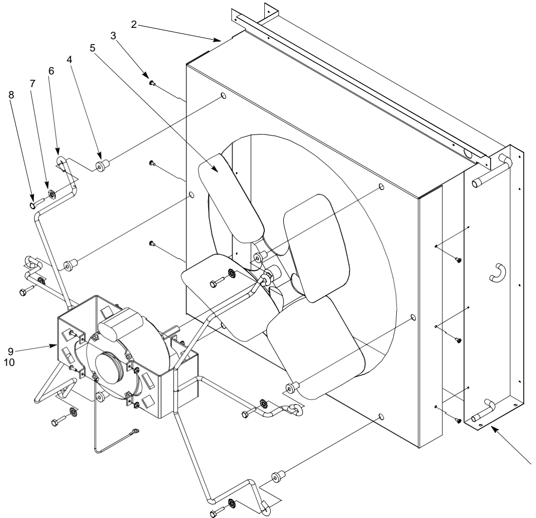
FIGURE 7. CONDENSER ASSEMBLY
