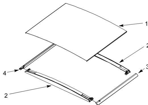
FIGURE 11. FRONT PANEL ASSEMBLY
