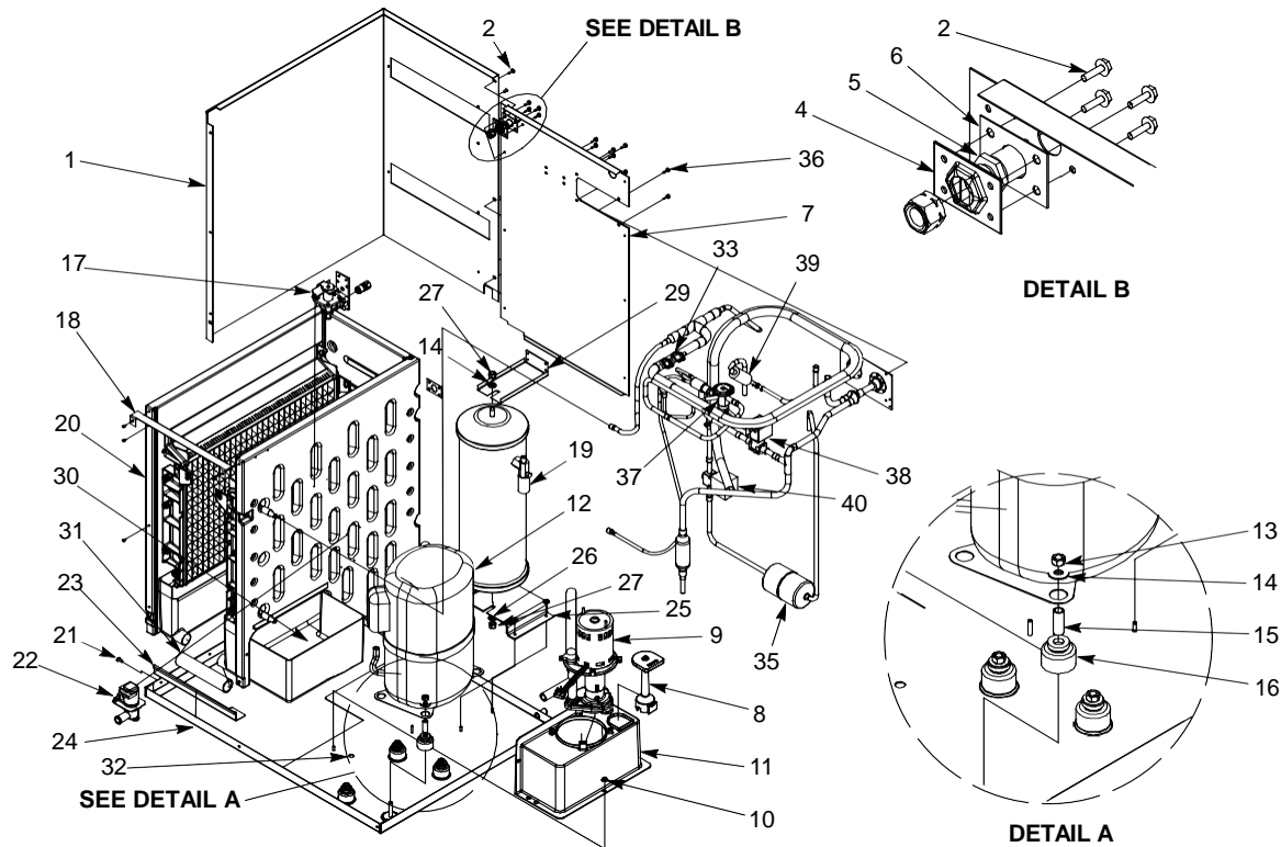
FIGURE 4. BUILD ASSEMBLY (REMOTE)
