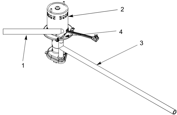
FIGURE 10. WATER PUMP ASSEMBLY
