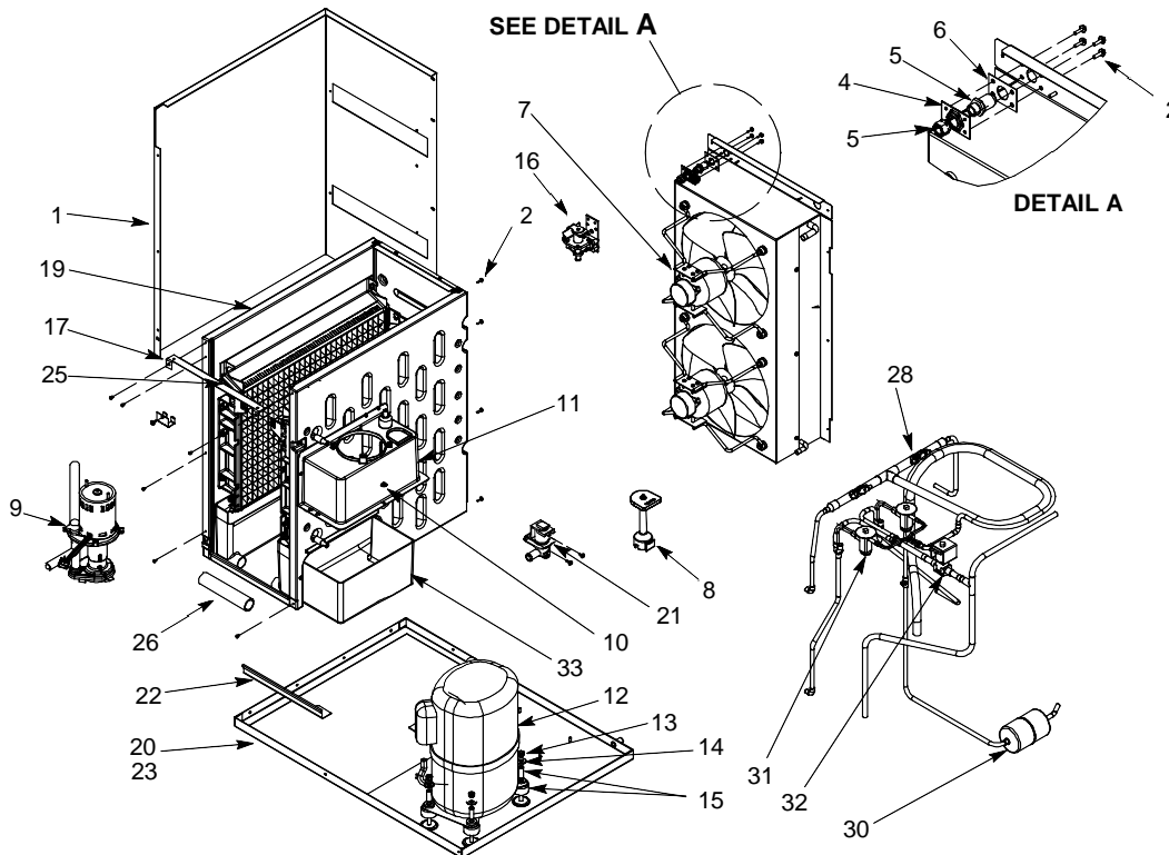
FIGURE 3. BUILD ASSEMBLY (AIR CONDENSER)
