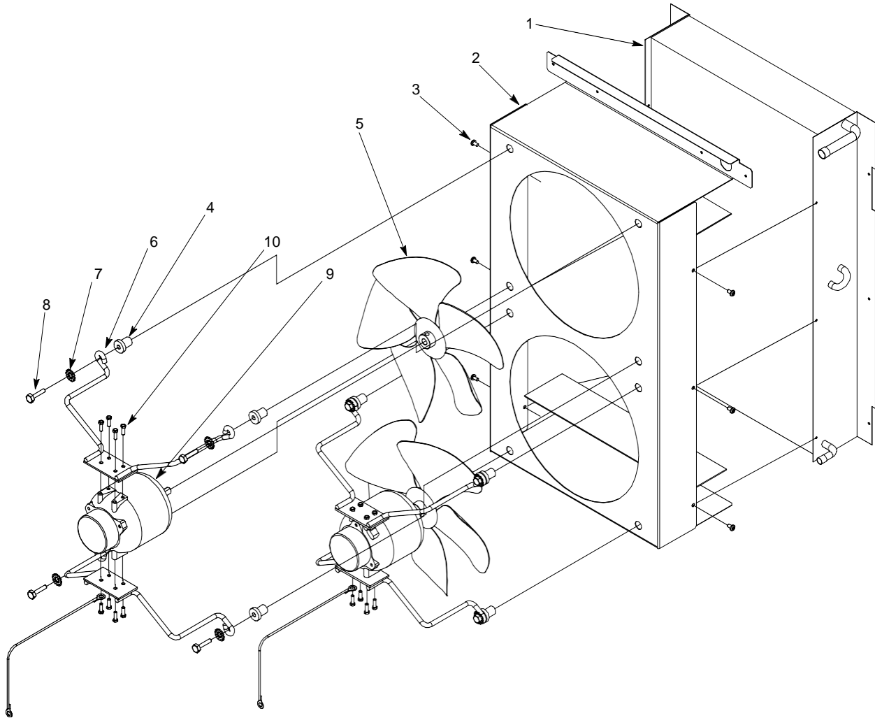
FIGURE 7. CONDENSER ASSEMBLY
