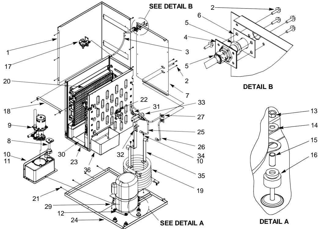
FIGURE 5. BUILD ASSEMBLY (WATER COOLED)
