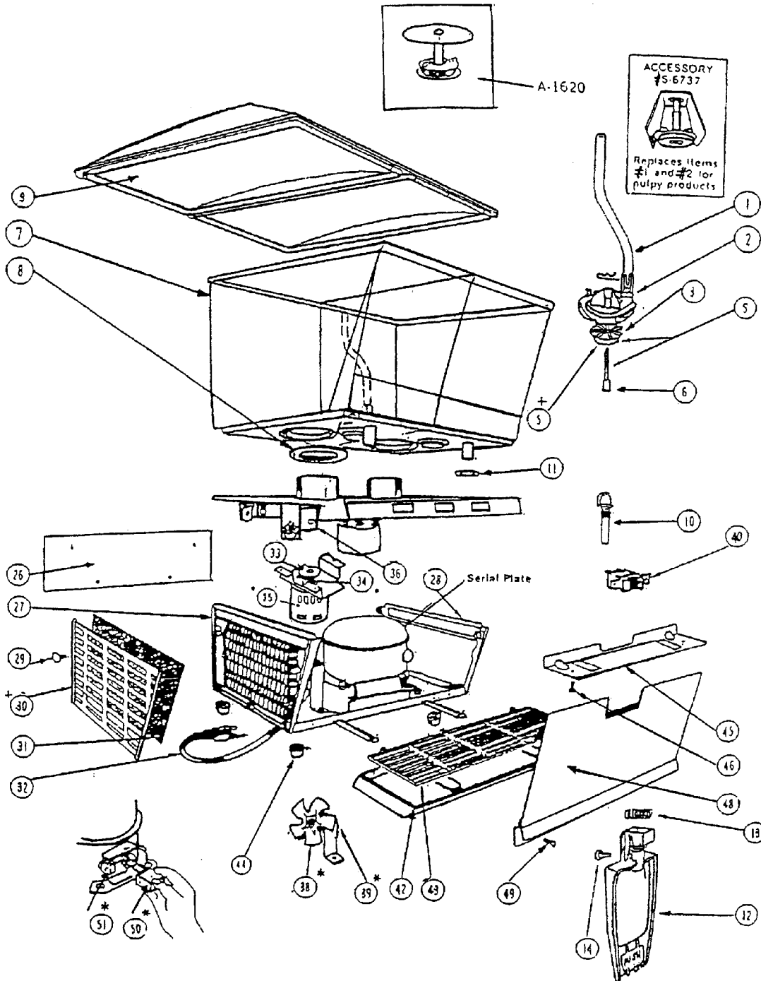
FIGURE 1. GENERAL ASSEMBLY
