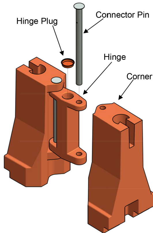
Corner Connector
