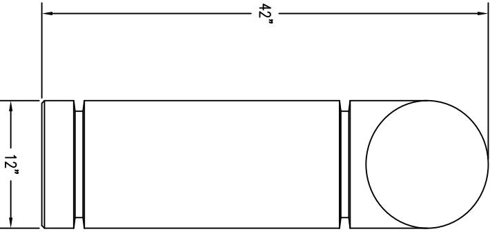
2 ELEVATION VIEW
