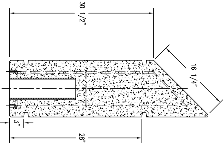
2 CROSS SECTION
