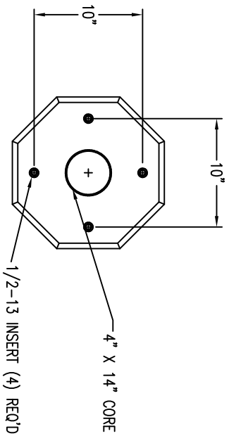
3 BOTTOM VIEW
