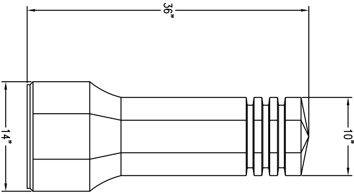
1 TOP VIEW
