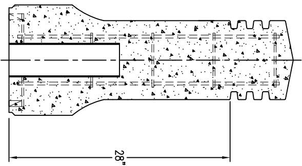
4 CROSS SECTION
