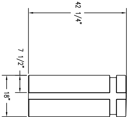
2 ELEVATION VIEW
