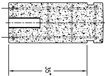
4 CROSS SECTION
