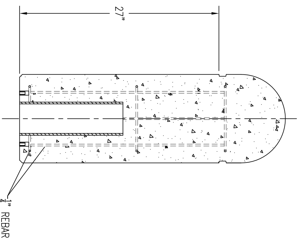
4 CROSS SECTION
