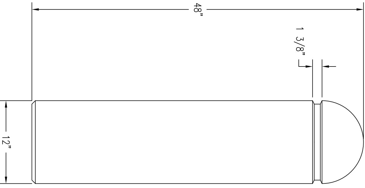
2 ELEVATION VIEW
