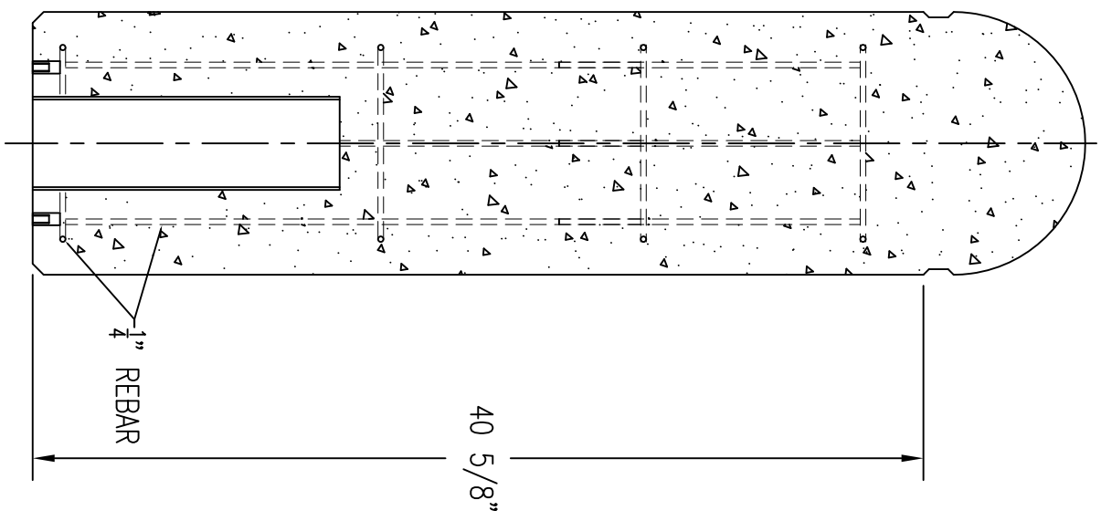
4 CROSS SECTION
