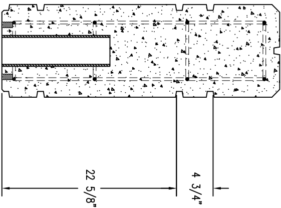
4 CROSS SECTION
