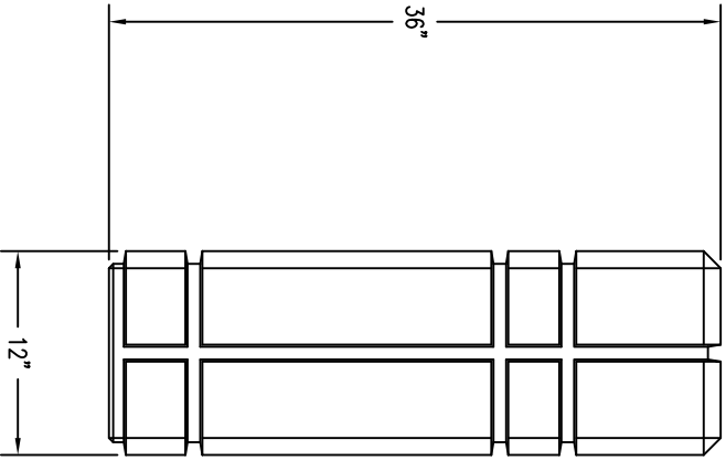
2 ELEVATION VIEW
